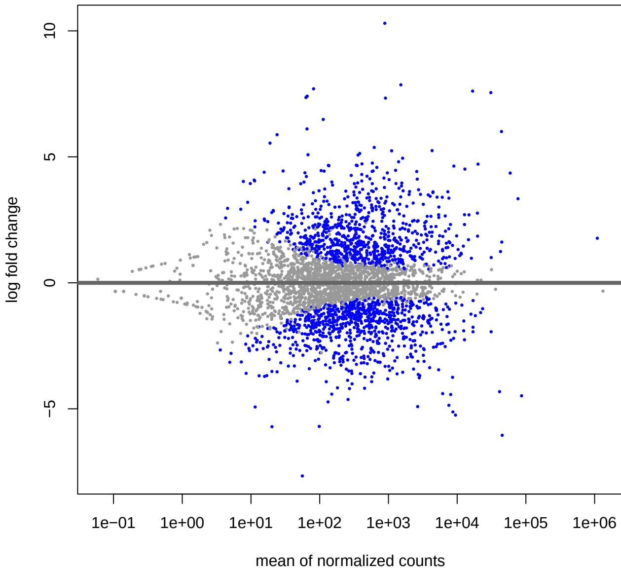
MA-plot for Growth_Media: Plate vs Broth
