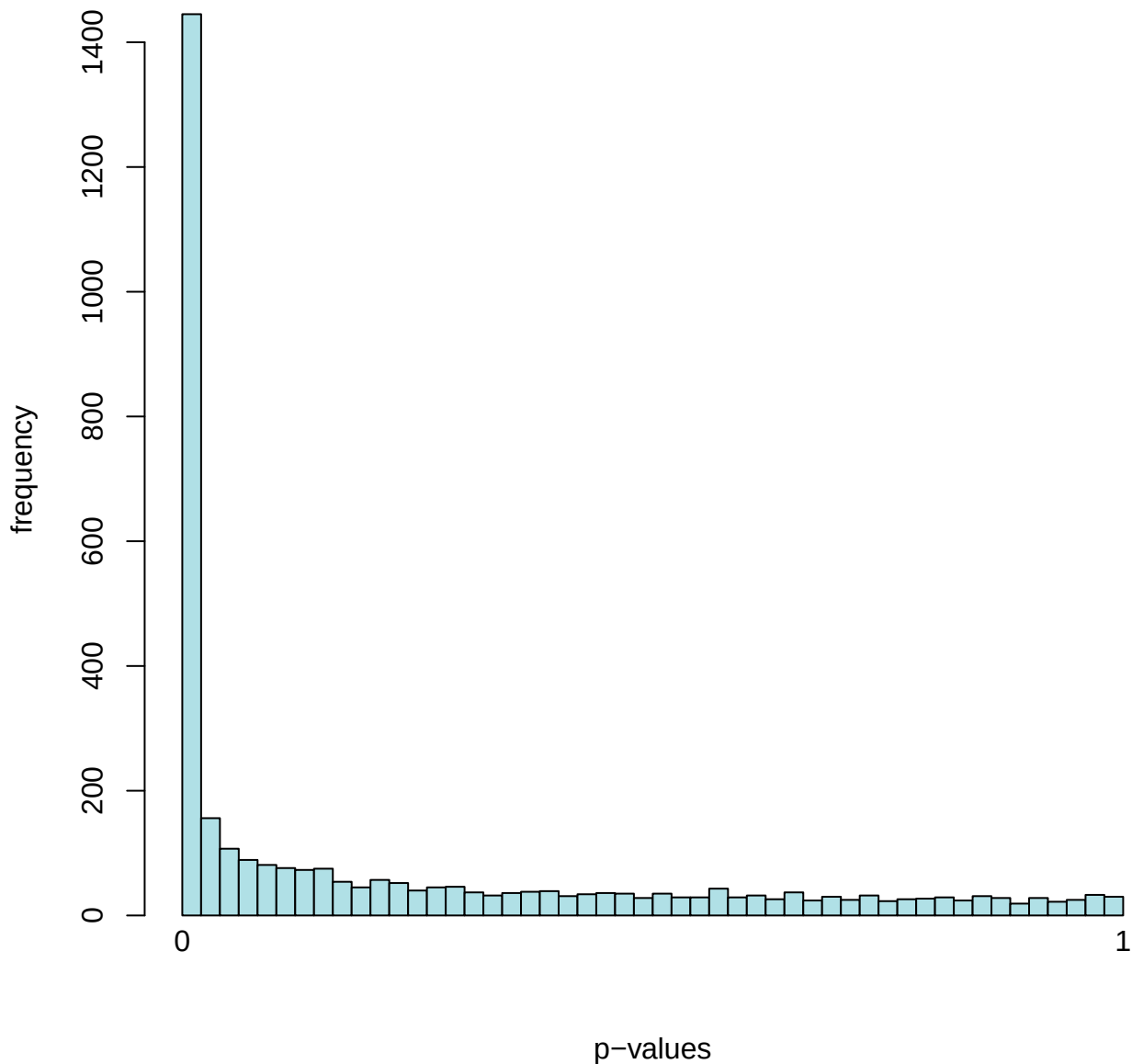
Histogram of p-values for Growth_Media: Plate vs Broth
